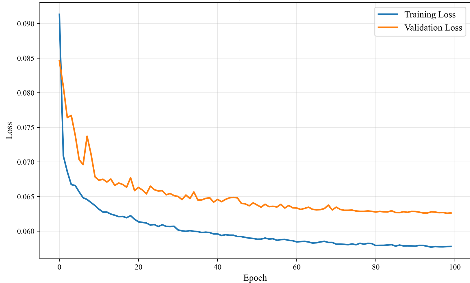
Bi-TSENet Training & Validation Loss - data4
